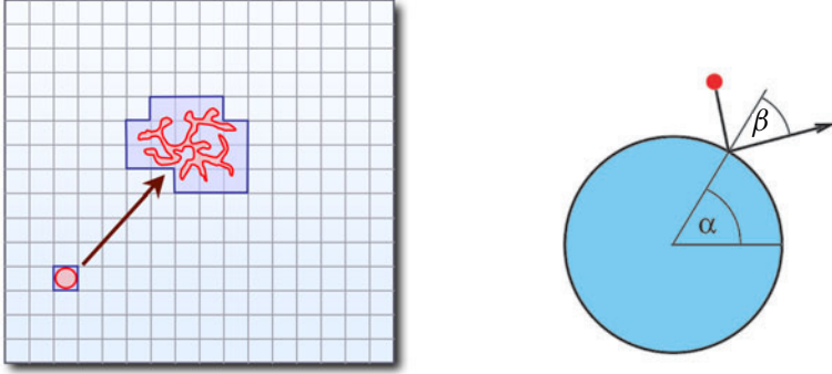
Figure 2. Left panel: Dispersion of a volume of initial conditions in phase space. Right panel: The Lorentz gas consists of a moving point particle that is elastically reflected when it collides with circular scatterers arranged on a regular triangular lattice. At the collision points, the state of the moving particle is specified by the two angles \alpha and \beta .
