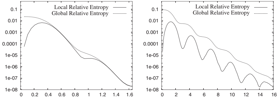
Figure 1. Time-decay of the H -function, in logarithmic scale, for the Boltzmann equation in one dimension of space and two dimensions of velocity, with periodic boundary conditions. The curve above is the H -function, the curve below is the purely kinetic part of the H -function; when the two curves are far from each other the gas is almost hydrodynamical, when they are close to each other it is almost homogeneous.
