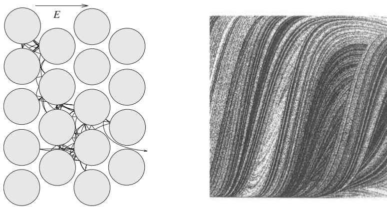
Figure 6. Left panel: Geometry and short trajectory of a periodic driven Lorentz gas. In addition to the elastic reflections, a constant force E and a Gauss thermostat acts on the wandering point particle. Right panel: Section of the phase-space probability in the stationary nonequilibrium state. The same coordinates as in Figure 3 are used.
