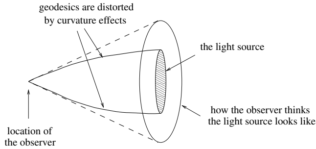
Figure 2. Because of positive curvature effects, the observer overestimates the surface of the light source.
