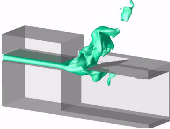
Figure 7. Complex air flow in a recorder as computed with the lattice Boltzmann method. Shown in green is an iso-speed surface at 40% of the maximum jet speed (simulation and figure by Helmut Kühnelt, University of Vienna).
