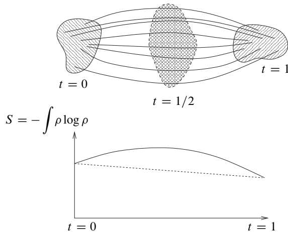
Figure 3. The lazy gas experiment: To go from initial state to final state, the lazy gas uses a path of least action. In a nonnegatively curved world, the trajectories of particles first diverge, then converge, so that at intermediate times the gas can afford to have a lower density (higher entropy).
