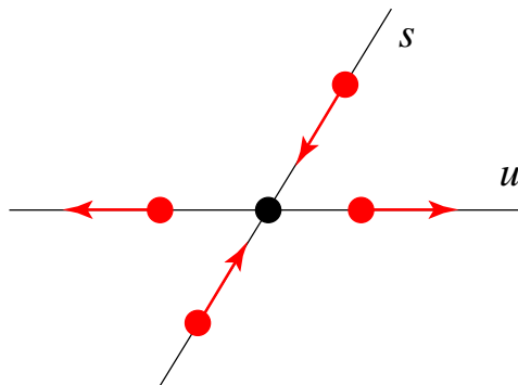
Figure 1. Unstable ( u ) and stable ( s ) manifolds associated with a phase point (thick bullet) in a two dimensional representation.
