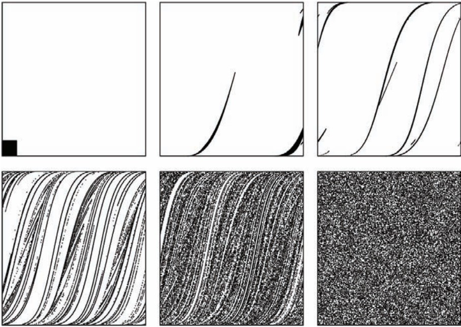
Figure 3. Spreading of initial conditions initially concentrated in a small part of the phase space of the Lorentz gas on a triangular lattice. Shown are sections of the phase space at the collisions of the moving particle with the replicated scatterer, where the angle \alpha is used on the x -axis and \sin \beta on the y -axis. The first plot in the upper left corner contains 100,000 points representing as many initial conditions. Subsequent plots correspond to phase space sections after 1, 2, 4, 6, and 10 collisions. The density of the scatterers is 4/5 of the close-packed density.
