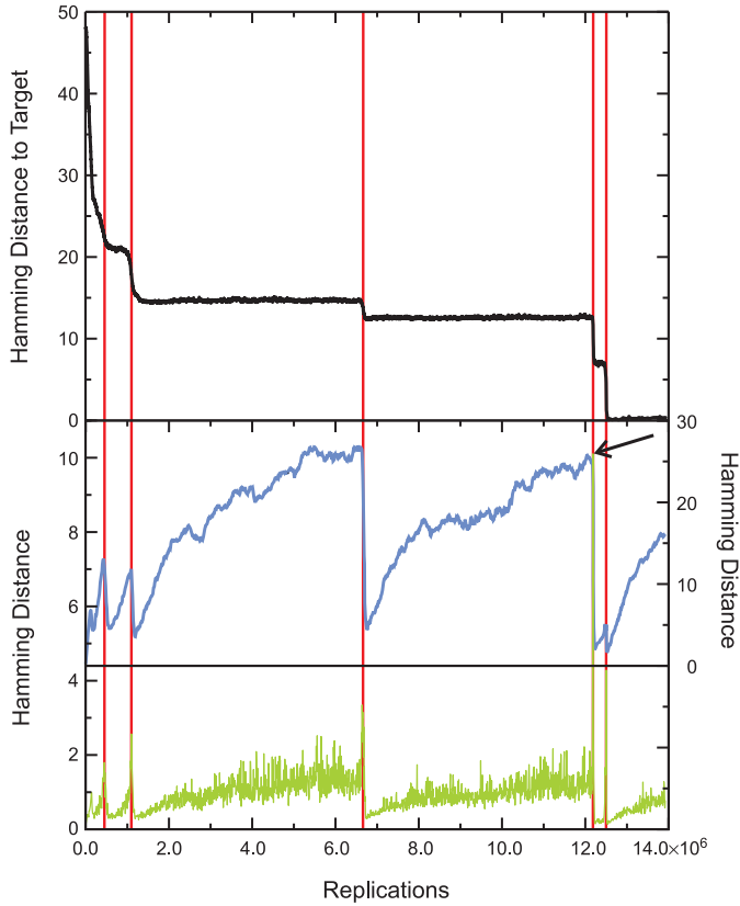
Figure 5. Evolutionary optimization of RNA structure. Shown is a single trajectory of a simulation of RNA optimization towards a tRNA phe target with population size n = 3000 and mutation rate p = 0.001 per site and replication. The figure shows as functions of time: (i) the distance to target averaged over the whole population, \overline{d_S(S_i, S_T)}(t) (black), (ii) the mean Hamming distance within the population, \overline{d_P}(t) (blue, right ordinate), and (iii) the mean Hamming distance between the populations at time t and t + \Delta t , \overline{d_C}(t, \Delta t) (green) with a time increment of \Delta t = 8000 . The end of plateaus (vertical red lines) are characterized by a collapse in the width of the population and a peak in the migration velocity corresponding to a jump in sequence space. The arrow indicates a remarkably sharp peak of d_C(t, 8000) around Hamming distance 10 at the end of the second long plateau ( t \approx 12.2 \times 10^6 replications). In other words, every adaptive phase is accompanied by a drastic reduction in genetic diversity, d_P(t) . The diversity increases during quasi-stationary epochs. On the plateaus the center of the cloud migrates only at a speed of Hamming distance 0.125 per 1000 replications.
